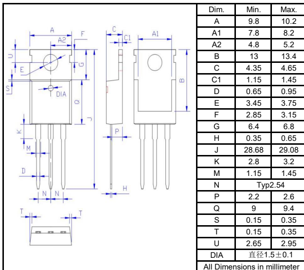
T0-220C
